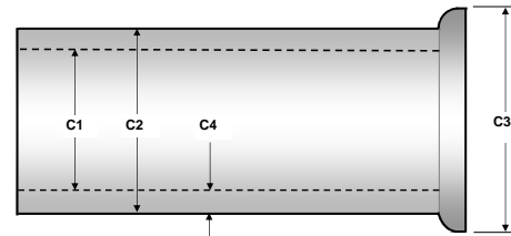
JOINT DETAILS
